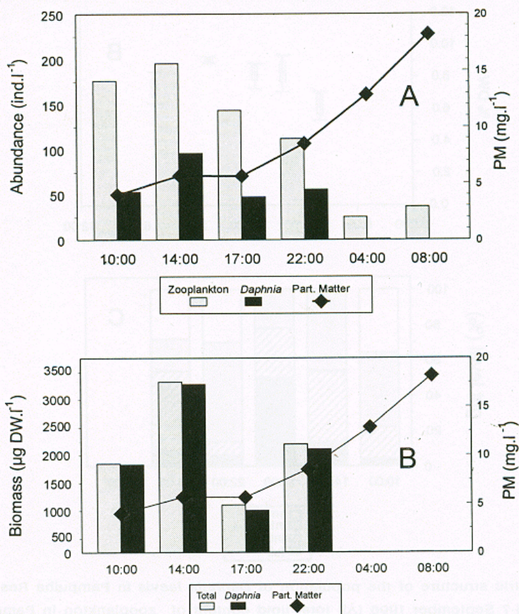
Figure 6: Temporal variations in the abundances of total zooplankton and Daphnia laevis . Suspended matter concentrations are also represented (A). Bottom: Total zooplankton and D. laevis biomass and suspended matter (B). All data refer to the diel cycle of 6-7 September 1996 in Pampulha Reservoir, Brazil.
