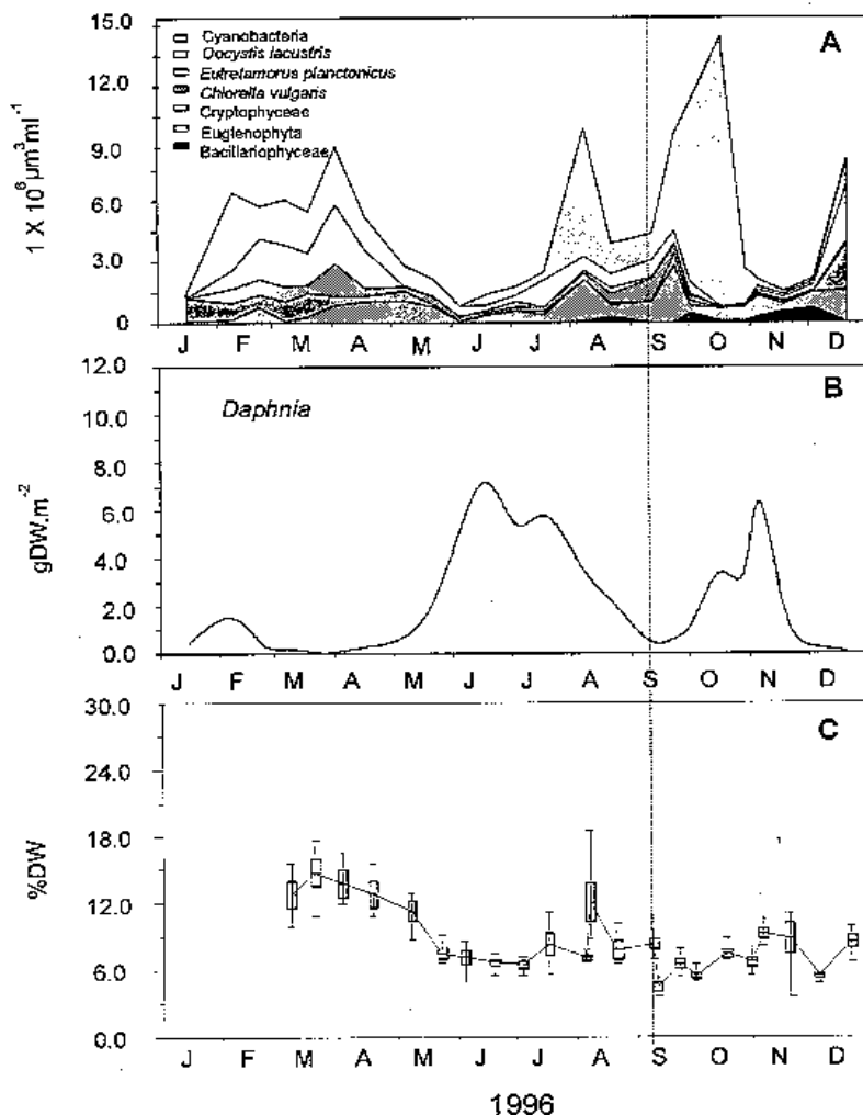
Figure 3: Annual course of phytoplankton biovolume (A), integrated biomass of Daphnia laevis (B) and total lipids of zooplankton in Pampulha Reservoir, 1996 (C). Only the most important groups of algae (in terms of biovolume) are here represented.
