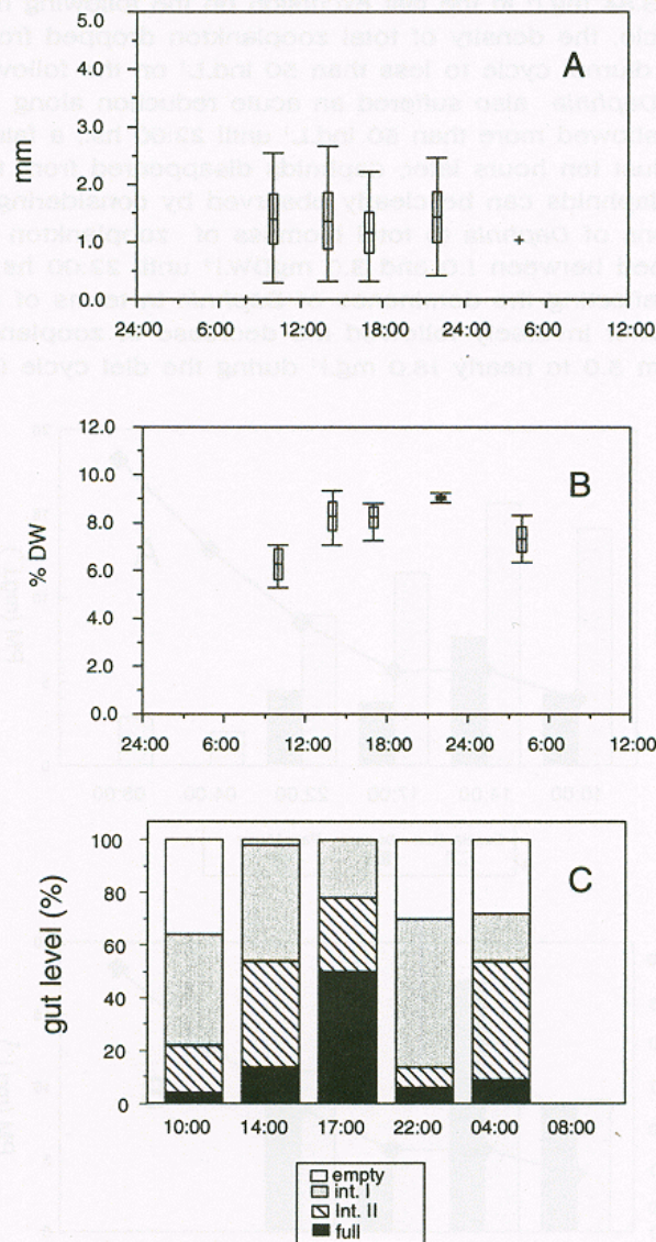
Figure 7: Allometric structure of the population of Daphnia laevis in Pampulha Reservoir from the diel cycle 6-7 September 1996 (A); total lipid content of zooplankton in Pampulha Reservoir (B). For plots A and B, mean, standard errors and ranges are given for each sample. Amount of food particles in the guts of D. laevis at different times of the day (C). At 4:00 hs am there was only a few individuals to perform the gut contents but the density as expressed by individuals per liter was negligible. All data refers to the diel cycle (6-7 September 1996) in Pampulha Reservoir.
